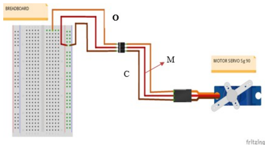
Gambar 3. 4 Rangkaian Motor Servo ke Breadboard
