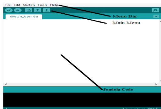
Gambar 2.2 Tampilan Arduino
