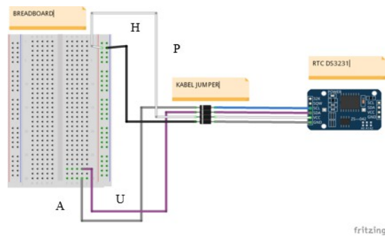
Gambar 3.3 Rangkaian RTC ke Breadboard
