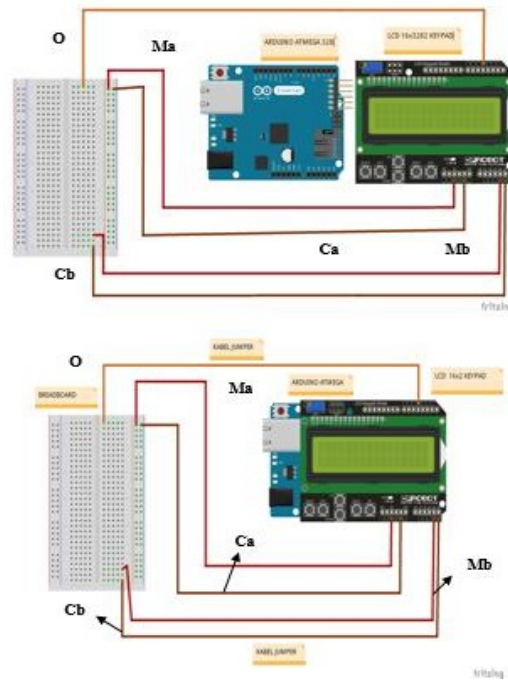
Gambar 3.5 Rangkaian LCD ke Breadboard
